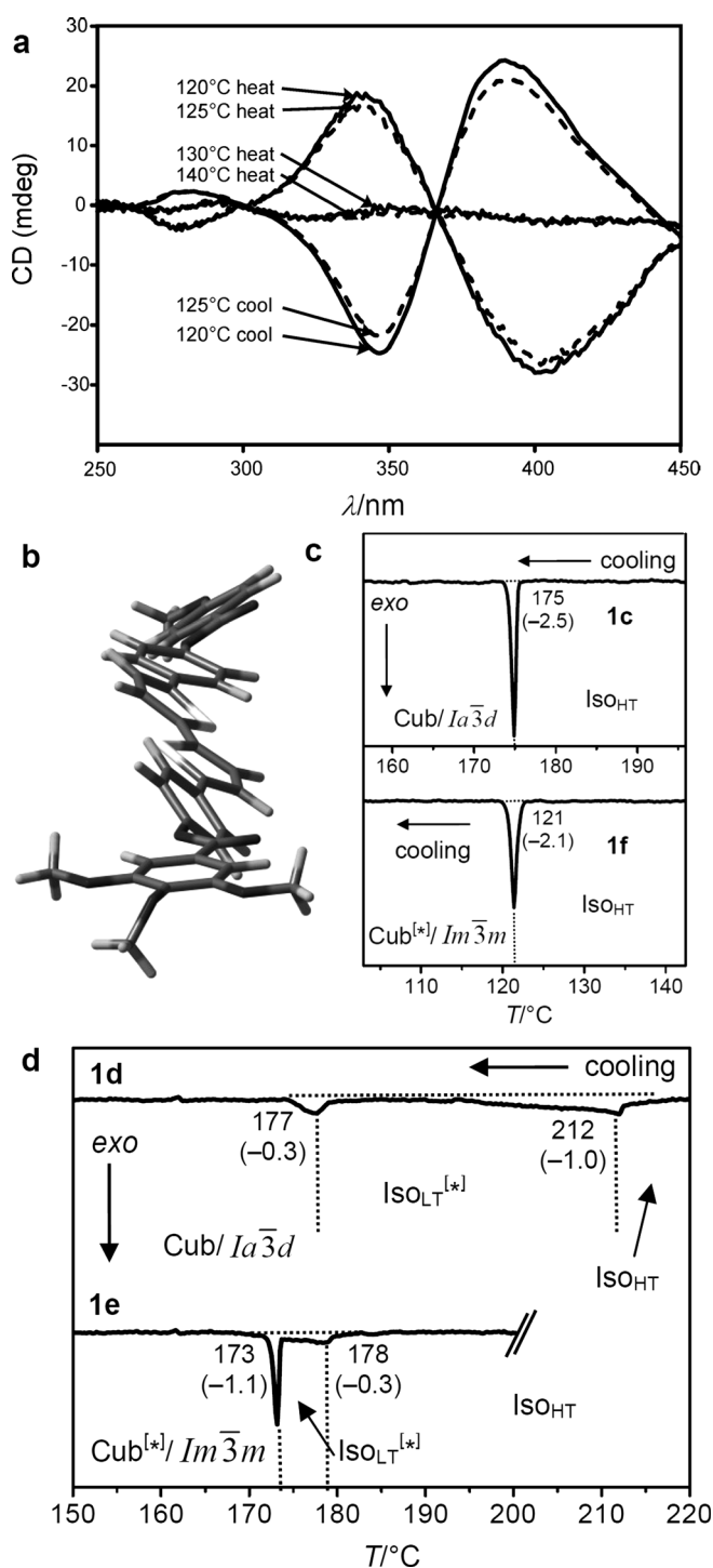
Figure 3. a) Temperature dependent CD spectra (ellipticity in mdeg) of a bulk film of compound 1g in the Cub [*] / Im \bar{3} m (120–125°C) and the Iso HT liquid (130–140°C). On cooling back to the Cub [*] / Im \bar{3} m (dashed curves) chirality reverses. b) Helical conformations as computed for a model compound related to compounds 1b,e with OCH 3 groups instead of the long alkyloxy chains. [23] c, d) DSC cooling thermograms of c) 1c and 1f with direct Iso HT –Cub transitions and d) 1d [23] and 1e with an intermediate Iso LT [*] phase (see also Figures S1–S6).
